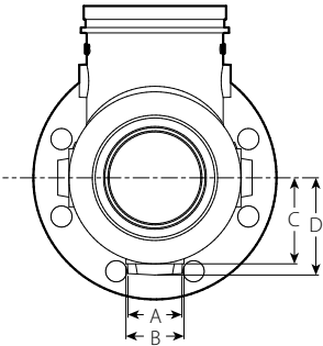
SERIES W731-D AGS SUCTION DIFFUSER – SUPPORT AND TAP BOSS LOCATION
